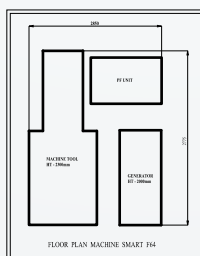
Floor Plan F64
